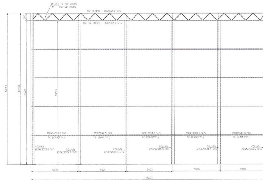
SIDE WALL ELEVATION ALONG GL - 1 & 5
