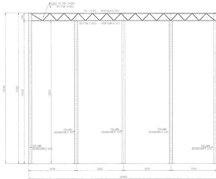
FRAME CROSS SECTION @ GL - A & F
