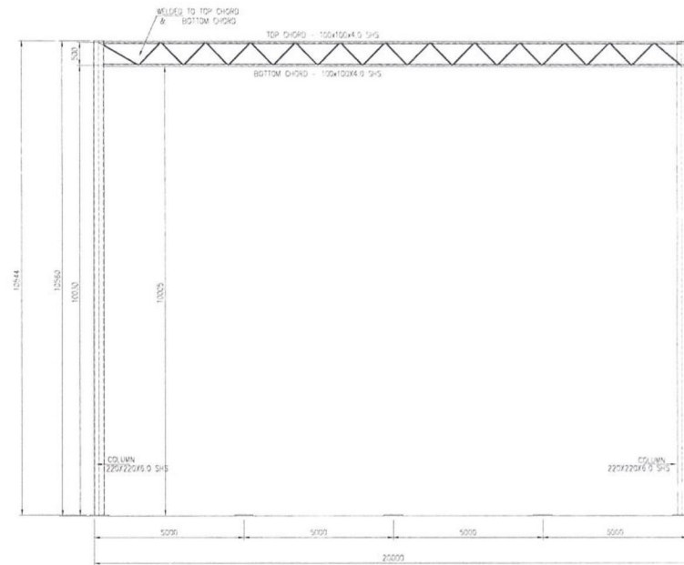
FRAME CROSS SECTION @ GL - B ~ E
